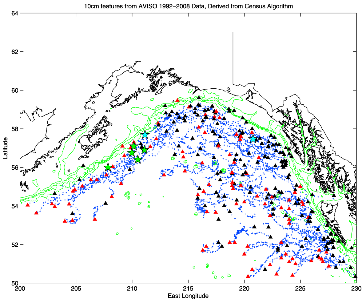
Figure 11. Start (black), end (red), and interim (blue) locations of feature centers from census algorithm. Cyan stars mark the start locations of the two features sampled, while the green stars mark the start locations of the other five Kenai eddies identified from altimetry. Clusters of feature formation are visible near the shelf in the Yakutat, Sitka, and Haida formation regions discussed previously. The 200, 500, 1000, and 2000 m isobaths are overlaid in green for reference.
