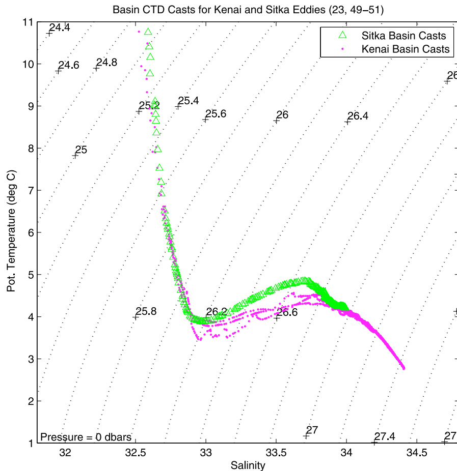
Figure 7. \theta -S properties for basin water from Sitka (green) and Kenai (magenta) CTD casts. The shape of the curves below a salinity of 32.7 is similar, with the magnitude of the temperature change in the 32.7–33.7 salinity range being \sim 1^\circ\text{C} , although the basin water near the Kenai Eddy is colder than that near the Sitka Eddy by \sim 0.3^\circ\text{C} over that salinity range.
