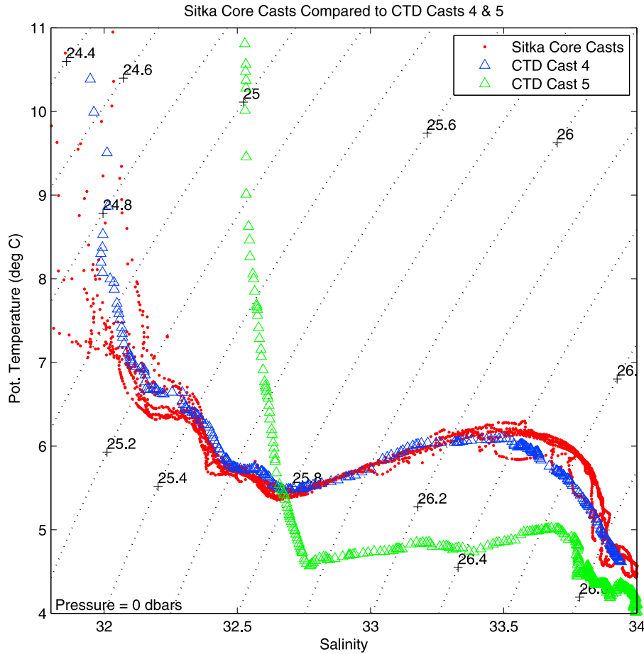
Figure 8. \theta - S Properties of Sitka Core water (red) with CTD Cast 4 (blue) and CTD Cast 5 (green) overlaid. The Core and CTD 4 curves are almost identical in the 32.3–33.5 salinity range and exhibit a maximum divergence of approximately 0.2–0.3°C in water saltier than 33.5, suggesting nearby formation.
