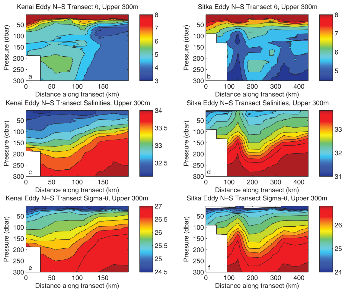
Figure 3. Profiles of (a, b) potential temperature, (c, d) salinity, and (e, f) potential density for the (a, c, e) Kenai and (b, d, f) Sitka eddies, moving from onshore (North) to offshore (South). Note that the temperature color axis has been truncated at 8^{\circ} in order to emphasize subsurface structure.
