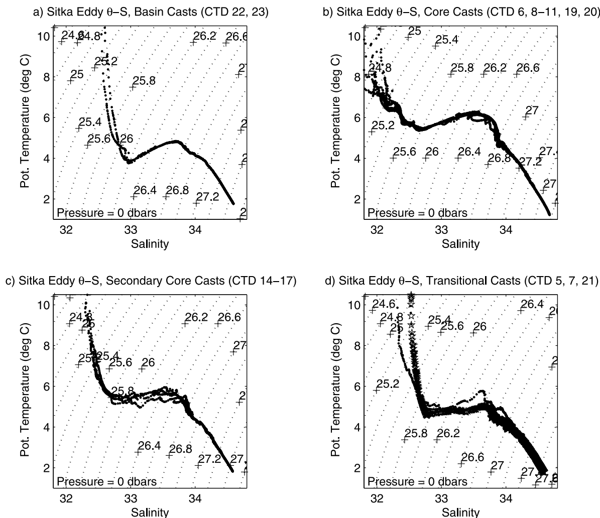
Figure 4. \theta -S diagrams for CTD casts from the (a) basin-like, (b) core-like, (c) secondary core-like, and (d) transitional groups for the Sitka Eddy. Groups were chosen based on a combination of \theta -S structural similarity and geographical location.
