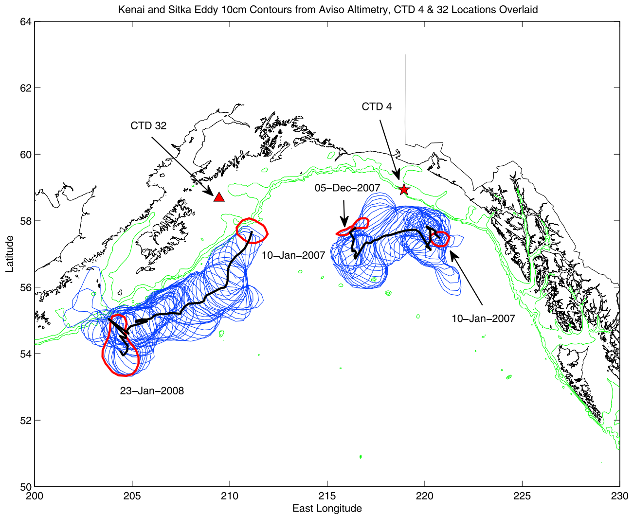
Figure 10. Weekly +10 cm SSHa contours for the Kenai and Sitka eddies, with starting and ending contours labeled and outlined in red and the trajectory of the eddy center overlaid in black. The locations of CTD casts 4 (red star) and 32 (red triangle) are overlaid. Bathymetry contours for 200, 500, and 1000 m of depth are shown in green.
