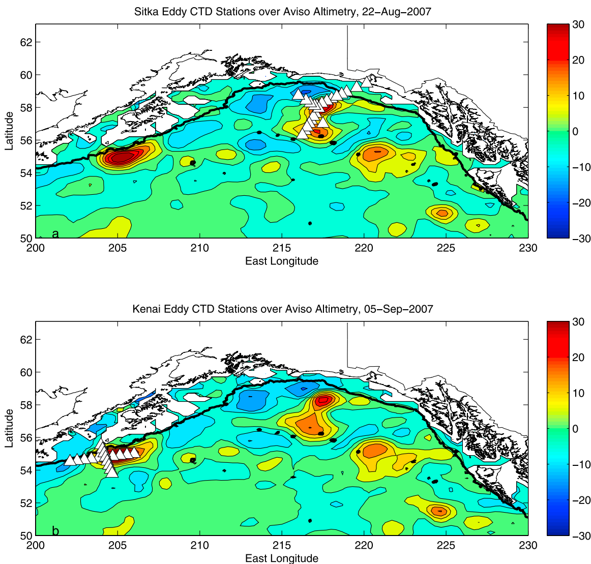
Figure 2. CTD cast locations for (a) the Sitka Eddy and (b) the Kenai Eddy, overlaid on 5 cm contours of SSHa from Aviso altimetry, with 1000 m isobath overlaid in thick black.
