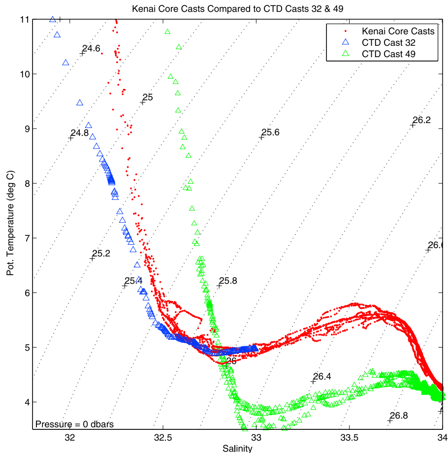
Figure 9. \theta -S properties of Kenai Core water (red) and CTD Cast 32 (blue), with basin CTD Cast 49 (green) overlaid for contrast. Although Cast 32 terminates at only 210 m of depth, the shape of the \theta -S curve below the surface layer (salinity greater than \sim 32.5 ) coincides almost exactly with that of the Kenai Core Casts. This suggests that the Kenai Eddy may have formed near the location of CTD Cast 32, on the shelf by the Kennedy and Stevenson entrances to Cooke Inlet.
