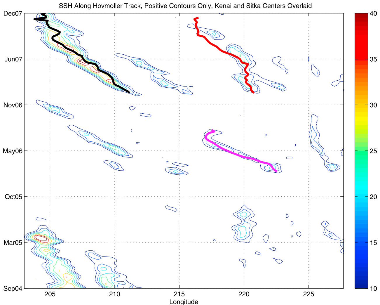
Figure 13. Positive SSHa Contours (5-cm interval, with first contour having a value of 10 cm) along center Hovmöller track, with Kenai (black) and Sitka (red) eddy center locations projected onto the track and overlaid. The earlier Sitka eddy mentioned in the text is also projected onto the track and overlaid in magenta.
