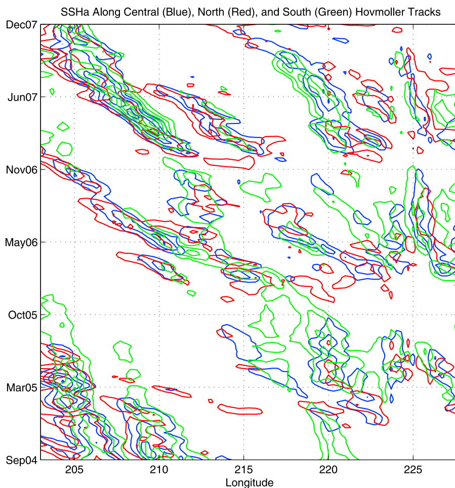
Figure 14. Positive SSHa contours (10-cm interval, with first contour having a value of 5 cm) along specified Hovmöller tracks: northern (red), center (blue), southern (green).
