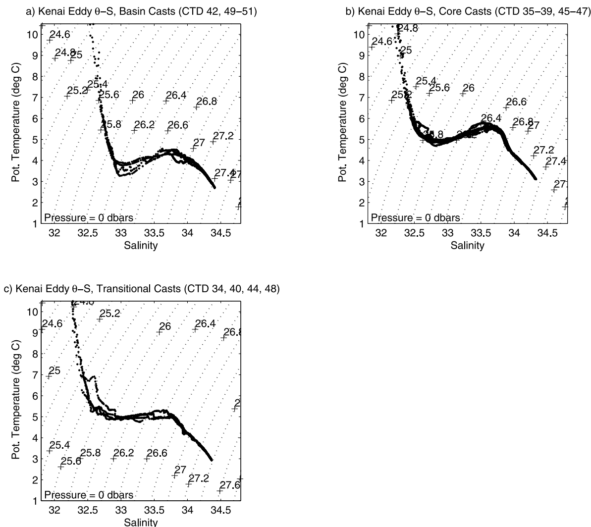
Figure 5. \theta -S properties by group for CTD casts from the (a) basin-like, (b) core-like, and (c) transitional groups for the Kenai Eddy. Groups were chosen based on a combination of structural similarity and geographical location relative to the Kenai Eddy.
