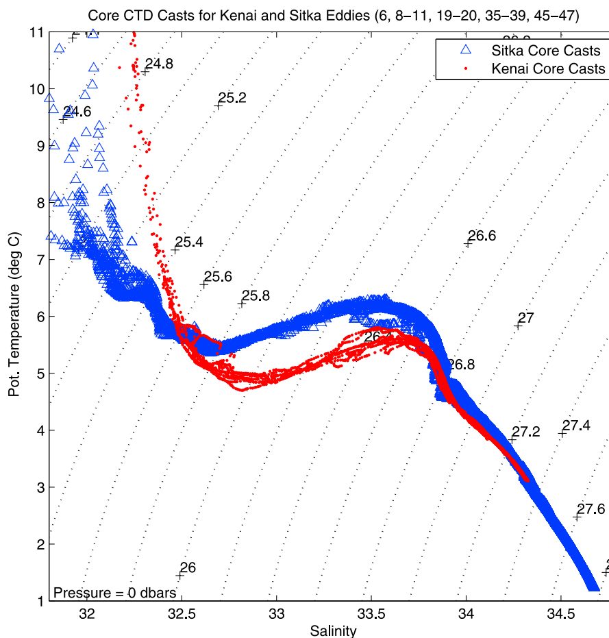
Figure 6. \theta -S properties for core water from Sitka (blue) and Kenai (red) CTD casts. The shape of the curves below a salinity of about 32.5 is similar, and the magnitude of the temperature change in the 32.6–33.6 range is \sim 1^\circ\text{C} in both cases. Note that the Kenai Core water over that salinity range is almost uniformly colder by \sim 1^\circ\text{C} .
